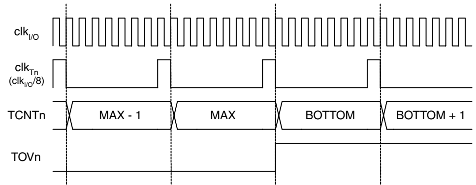
Figure 60. Timer/Counter Timing Diagram, with Prescaler ( f_{\text{clk\_I/O}}/8 )
