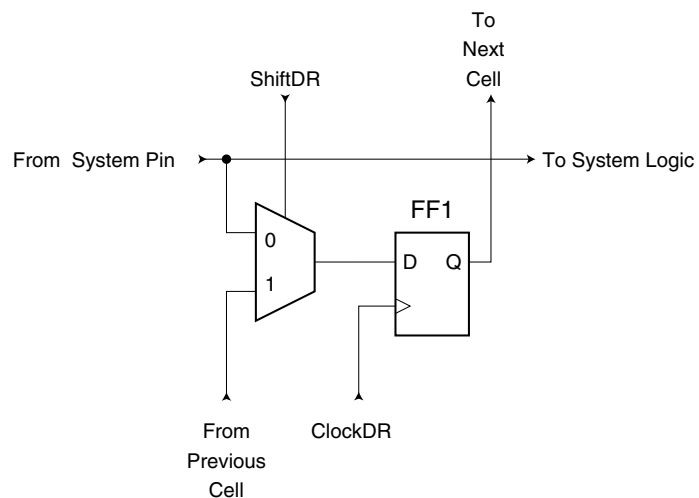
Figure 110. Observe-only Cell
